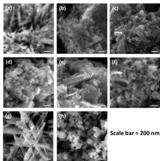
Figure 3. Scanning electron microscope (SEM) images of the eight Mn oxides reported herein: (a) \beta -MnO 2 , (b) R-MnO 2 , (c) \alpha -MnO 2 , (d) \delta -MnO 2 , (e) \lambda -MnO 2 , (f) LiMn 2 O 4 , (g) Mn 2 O 3 , and (h) Mn 3 O 4 .
