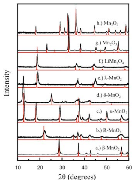
Figure 2. Powder X-ray diffraction patterns of the eight Mn oxides reported herein: (a) \beta -MnO 2 , (b) R-MnO 2 , (c) \alpha -MnO 2 , (d) \delta -MnO 2 , (e) \lambda -MnO 2 , (f) LiMn 2 O 4 , (g) Mn 2 O 3 , and (h) Mn 3 O 4 . The sample patterns (black) agree with the reference (red) in all cases except (e) where the reference shown is for LiMn 2 O 4 and the observed shift is indicative of delithiation forming \lambda -MnO 2 .
