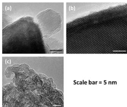
Figure 5. High-resolution transmission electron microscope (HRTEM) images of the three active water oxidation Mn oxides post reaction: (a) Mn 3 O 4 , (b) Mn 2 O 3 , (c) \lambda -MnO 2 . See Supporting Information for survey.
